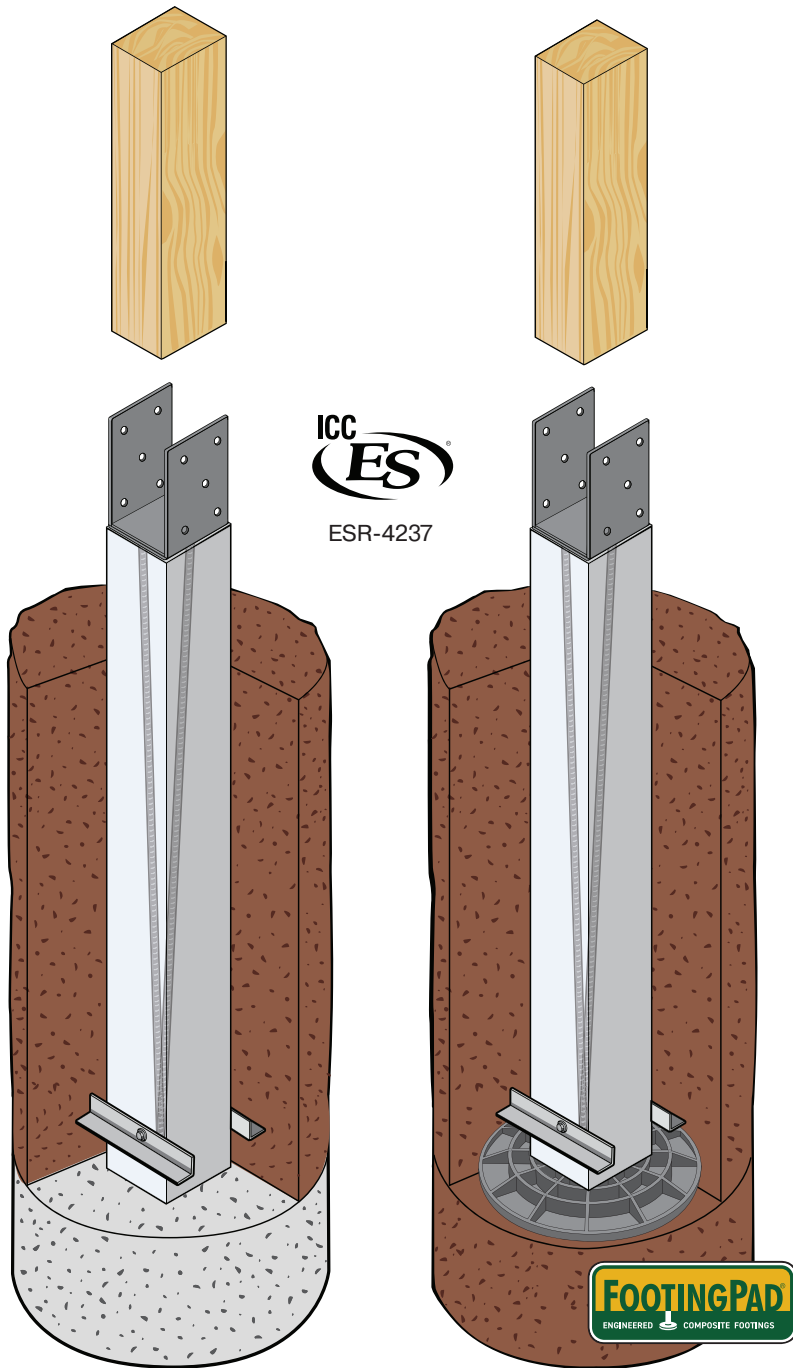
Precast concrete footer with uplift anchors
